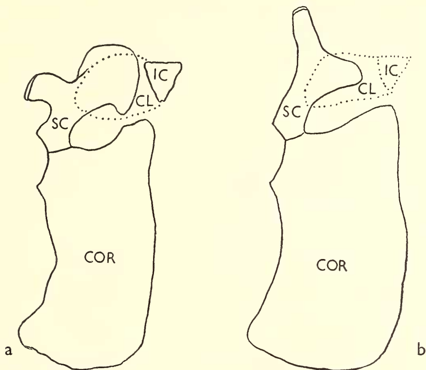
TEXT-FIG. 2. Pectoral girdles in dorsal view. a , Peloneustes philarchus (Seeley), \times \frac{1}{5} , from Andrews. b , Pliosaurus macromerus Phillips, \times \frac{1}{16} . CL., Clavicle; COR., Coracoid; IC., Interclavicle; SC., Scapula. Dotted lines indicate possible position of clavicular arch.
